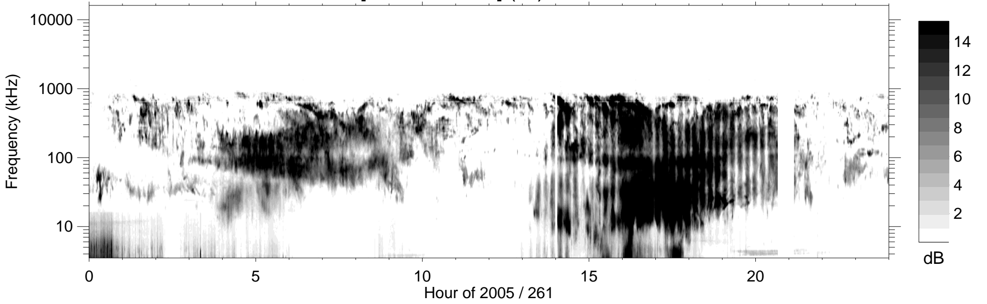
RPWS [ABCH1H2/Ex] (-B) 2005/09/18
