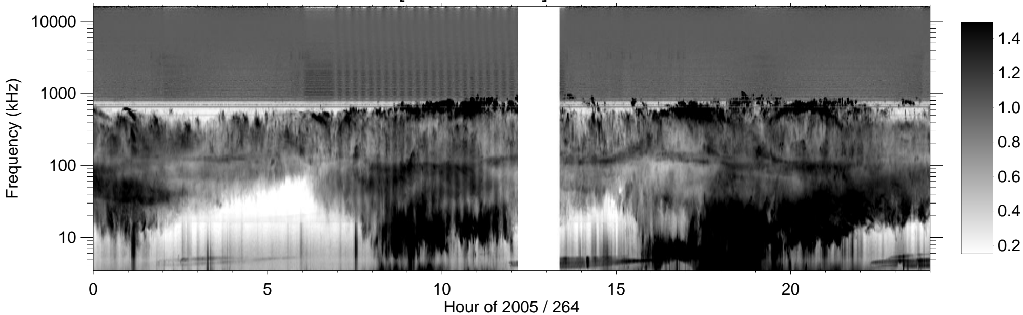
RPWS [ABCH1H2/Ex] (-B) 2005/09/21
