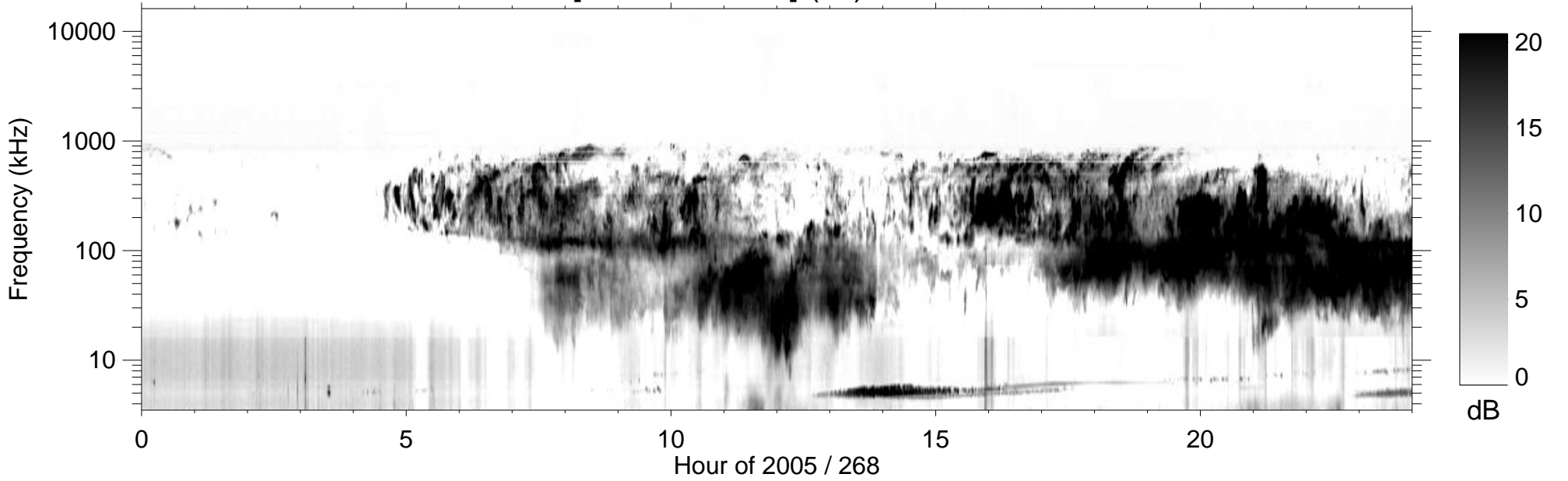
RPWS [ABCH1H2/Ex] (-B) 2005/09/25
