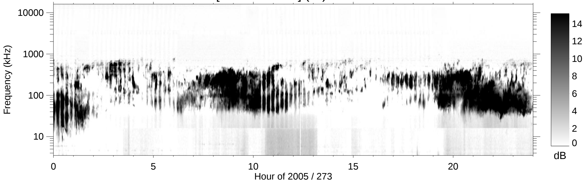
RPWS [ABCH1H2/Ex] (-B) 2005/09/30
