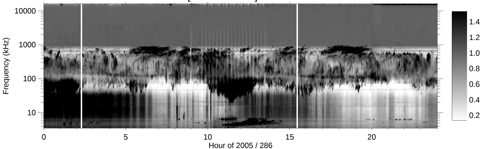
RPWS [ABCH1H2/Ex] (-B) 2005/10/13
