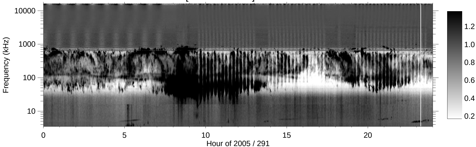
RPWS [ABCH1H2/Ex] (-B) 2005/10/18
