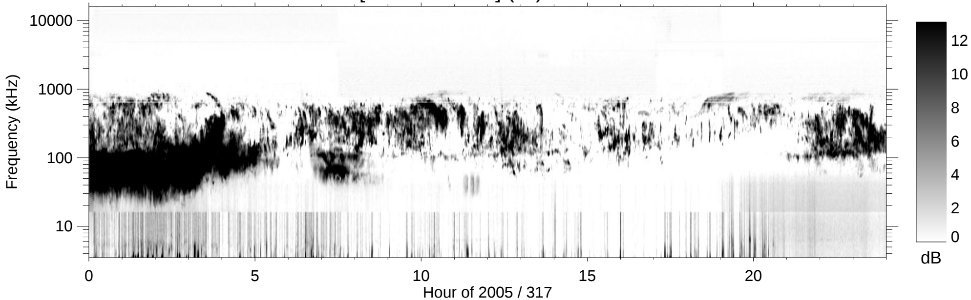
RPWS [ABCH1H2/Ex] (-B) 2005/11/13
