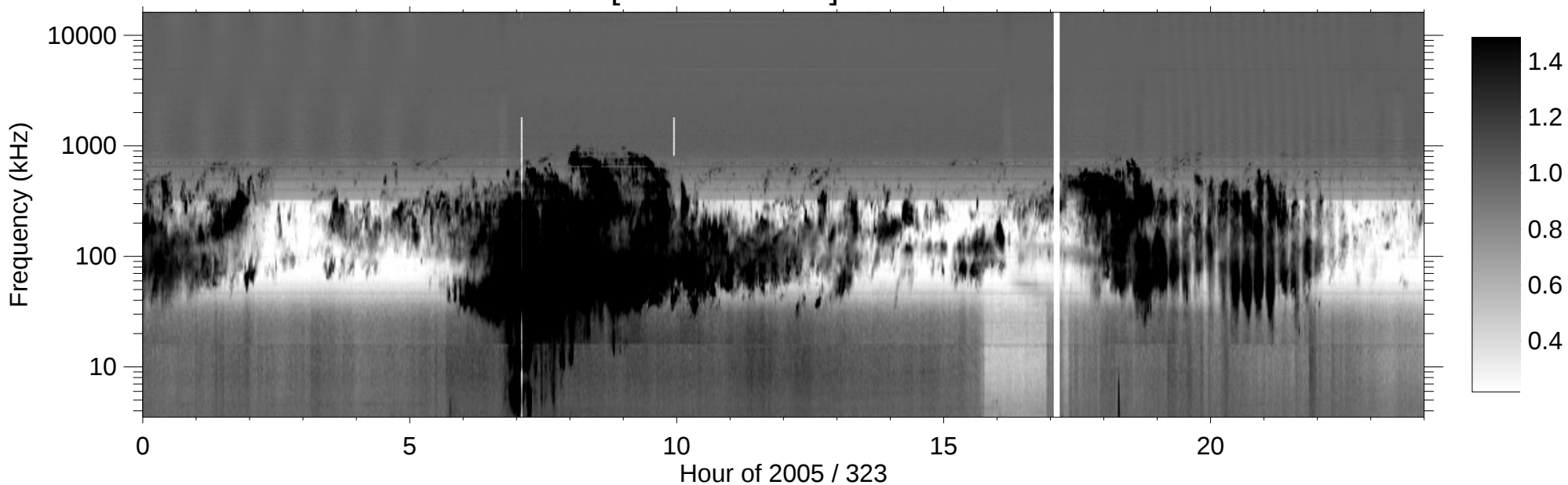
RPWS [ABCH1H2/Ex] (-B) 2005/11/19
