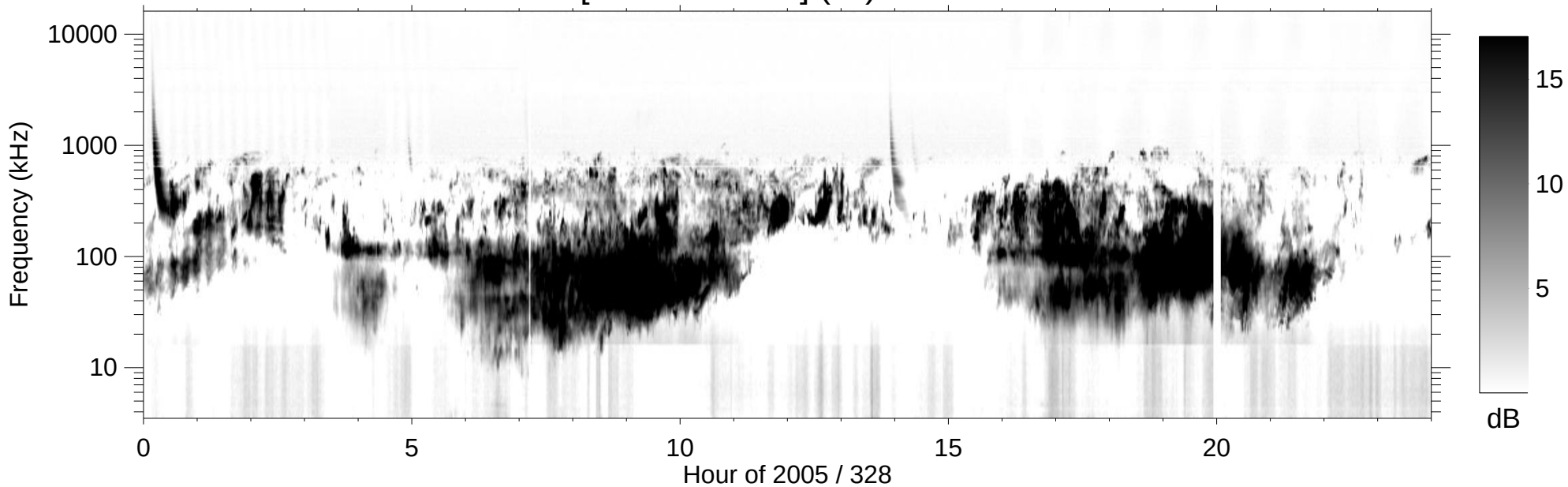
RPWS [ABCH1H2/Ex] (-B) 2005/11/24
