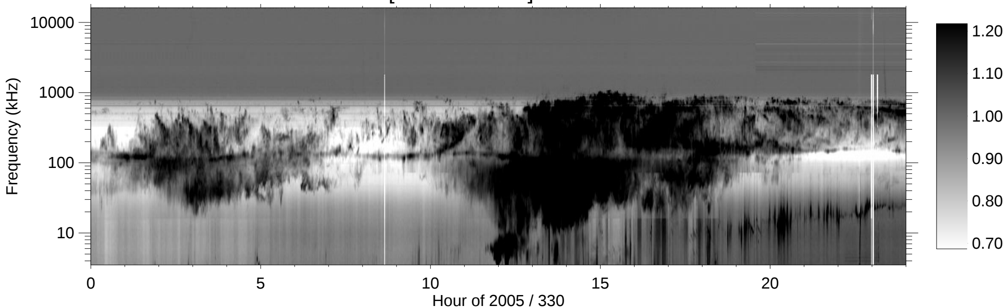
RPWS [ABCH1H2/Ex] (-B) 2005/11/26
