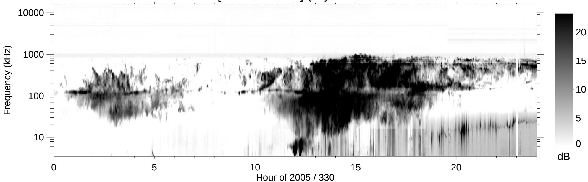
RPWS [ABCH1H2/Ex] (-B) 2005/11/26
