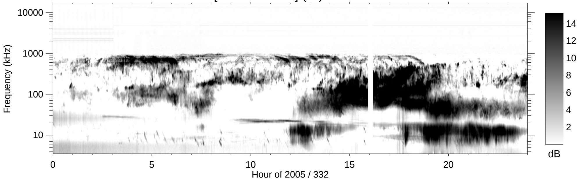
RPWS [ABCH1H2/Ex] (-B) 2005/11/28
