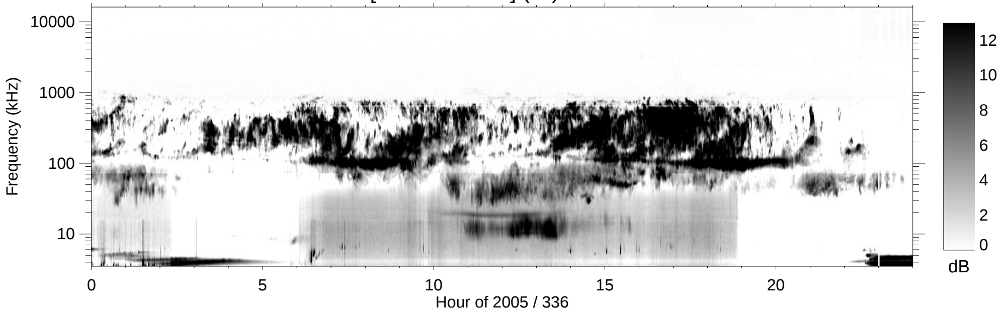
RPWS [ABCH1H2/Ex] (-B) 2005/12/02
