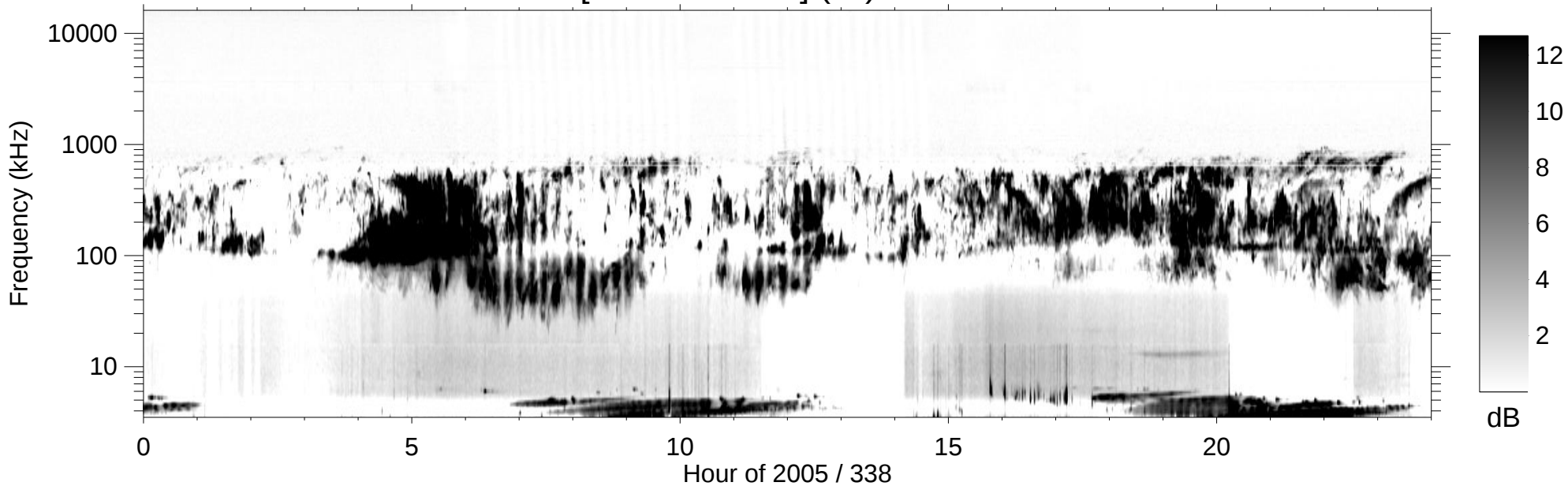
RPWS [ABCH1H2/Ex] (-B) 2005/12/04
