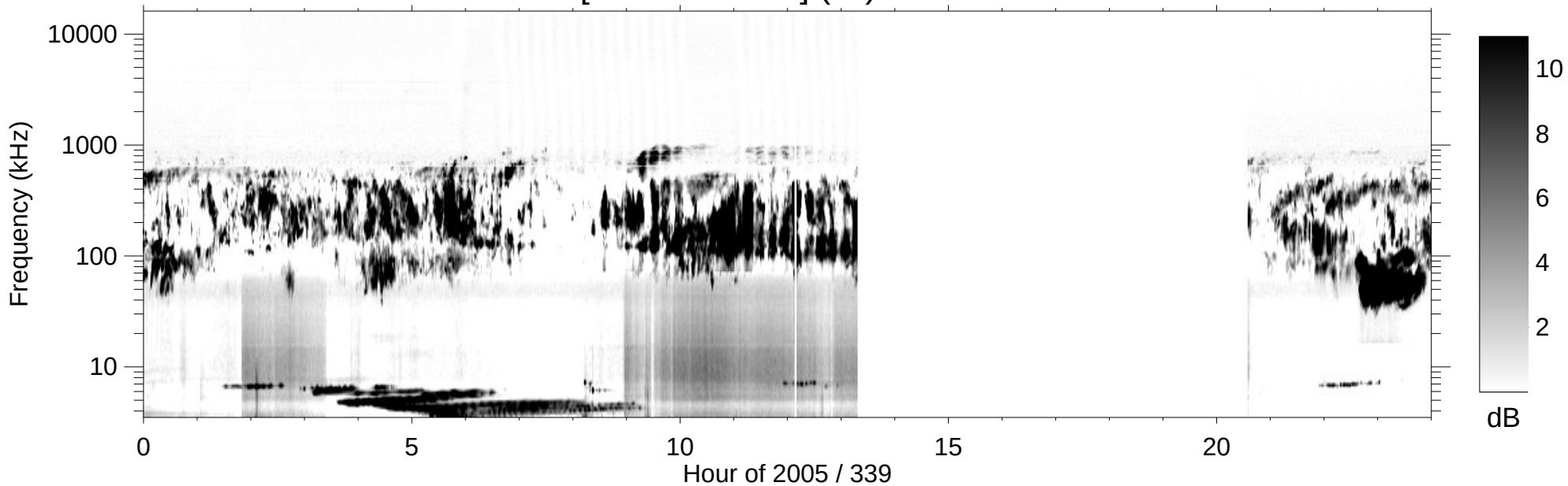
RPWS [ABCH1H2/Ex] (-B) 2005/12/05
