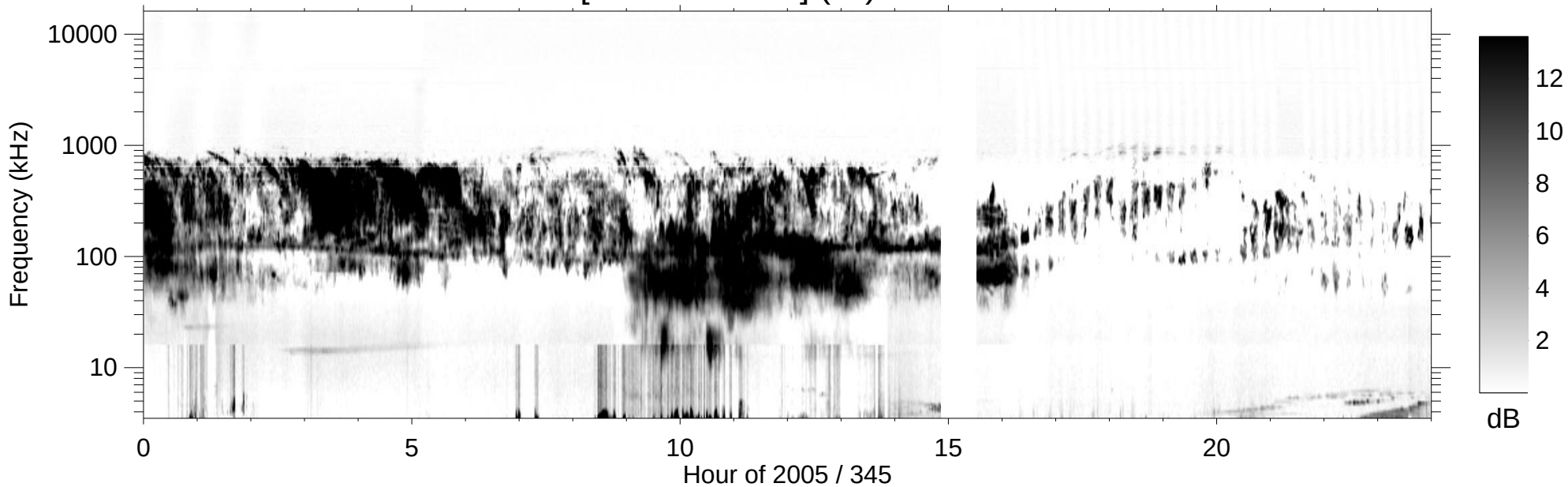
RPWS [ABCH1H2/Ex] (-B) 2005/12/11
