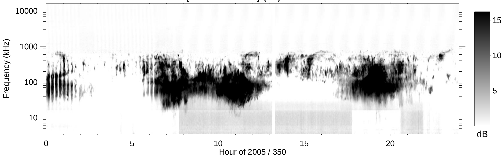
RPWS [ABCH1H2/Ex] (-B) 2005/12/16
