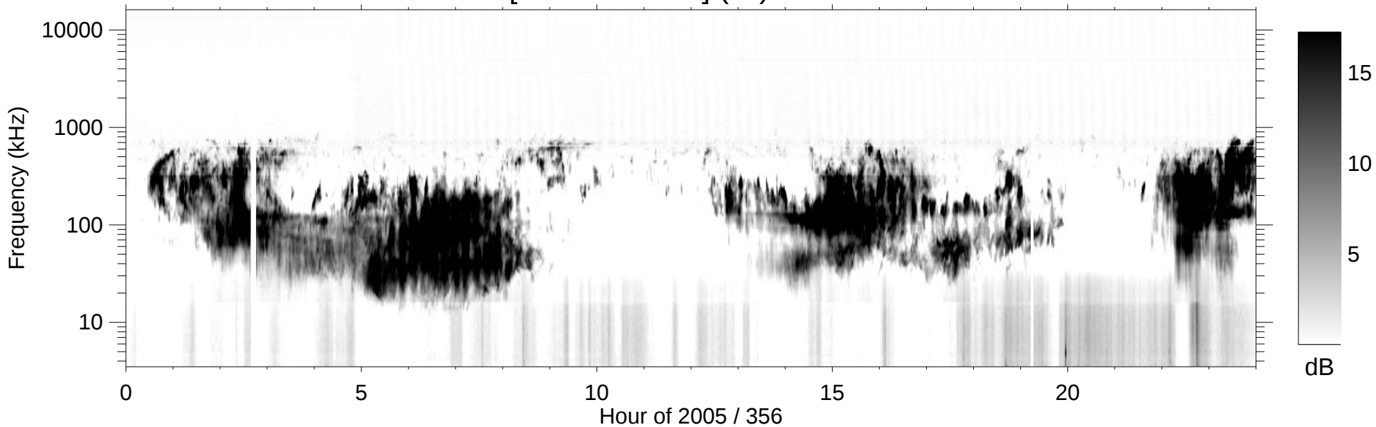
RPWS [ABCH1H2/Ex] (-B) 2005/12/22
