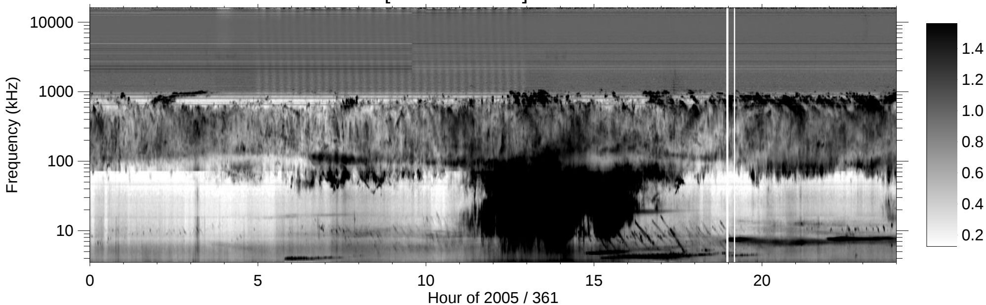
RPWS [ABCH1H2/Ex] (-B) 2005/12/27
