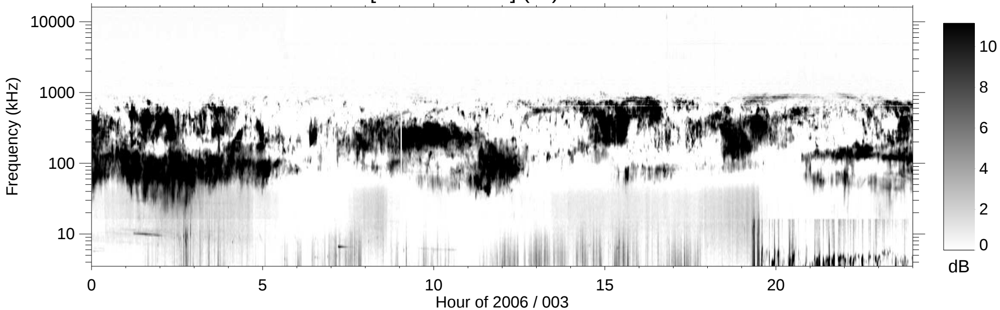
RPWS [ABCH1H2/Ex] (-B) 2006/01/03
