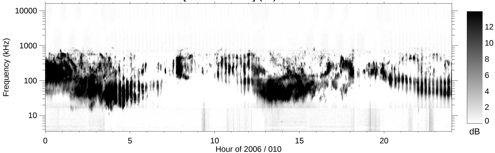
RPWS [ABCH1H2/Ex] (-B) 2006/01/10
