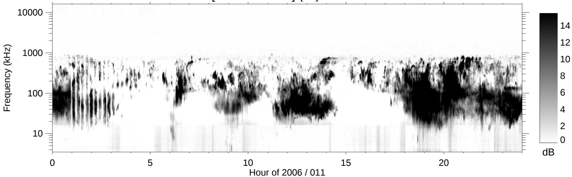
RPWS [ABCH1H2/Ex] (-B) 2006/01/11
