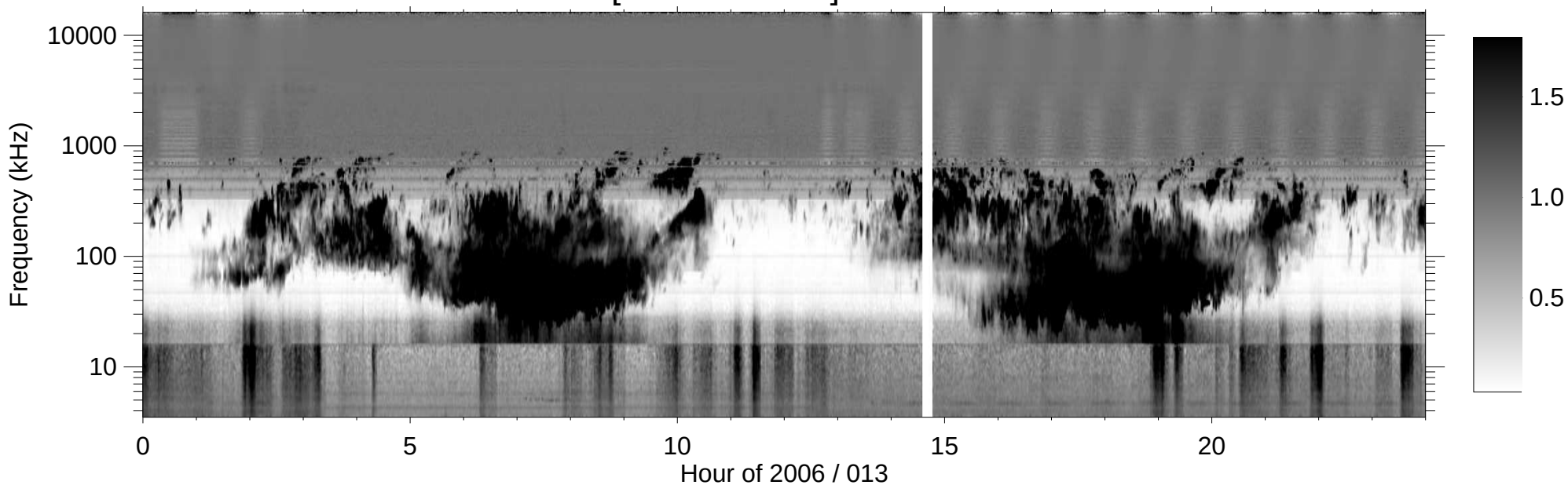
RPWS [ABCH1H2/Ex] (-B) 2006/01/13
