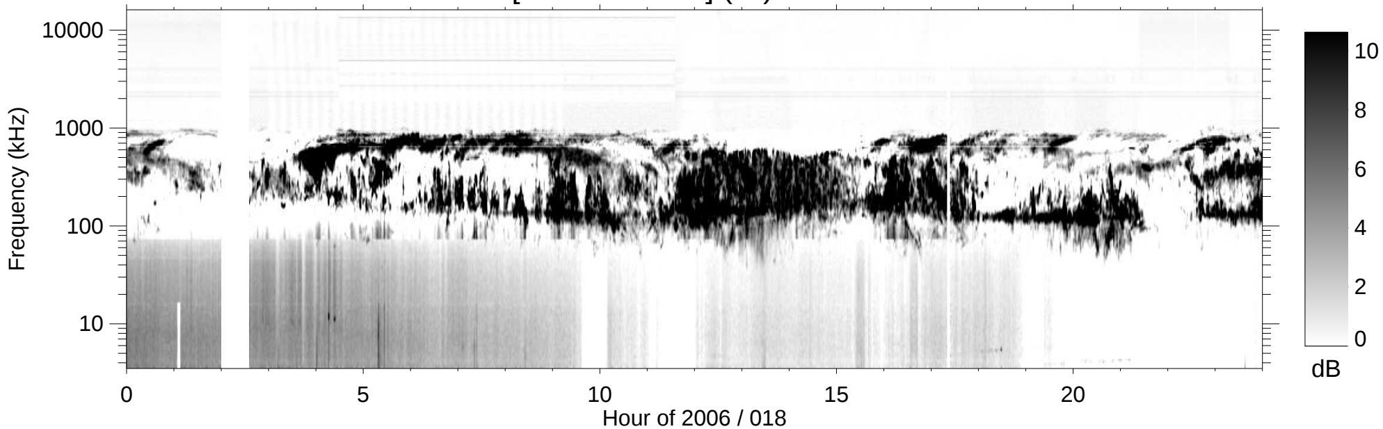
RPWS [ABCH1H2/Ex] (-B) 2006/01/18
