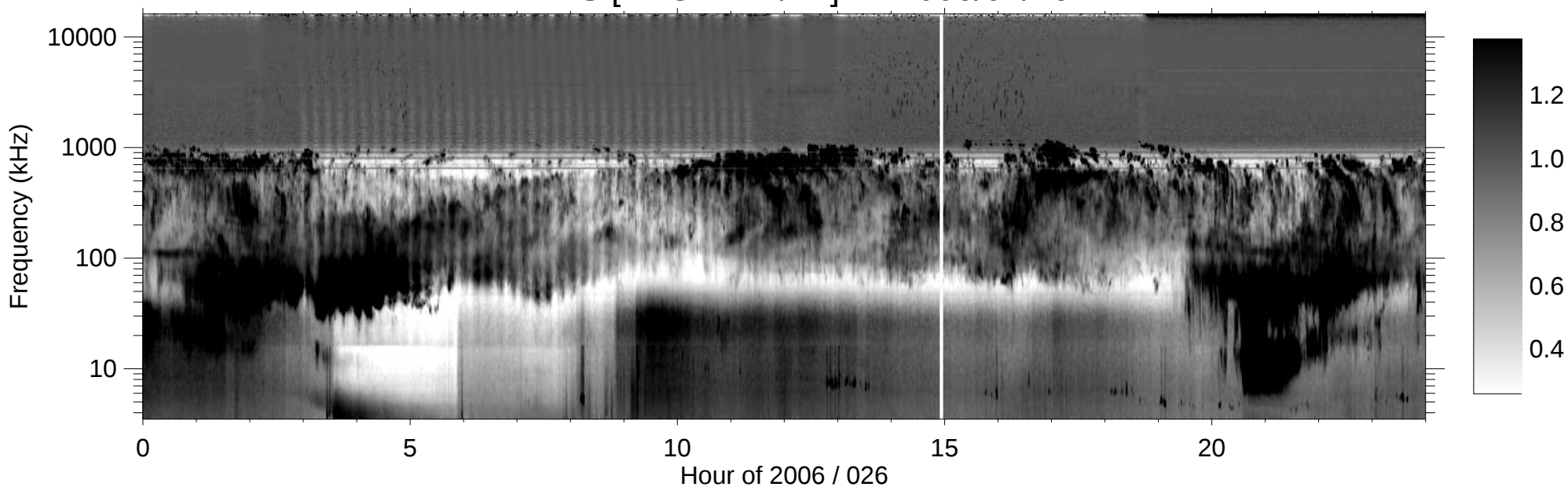
RPWS [ABCH1H2/Ex] (-B) 2006/01/26
