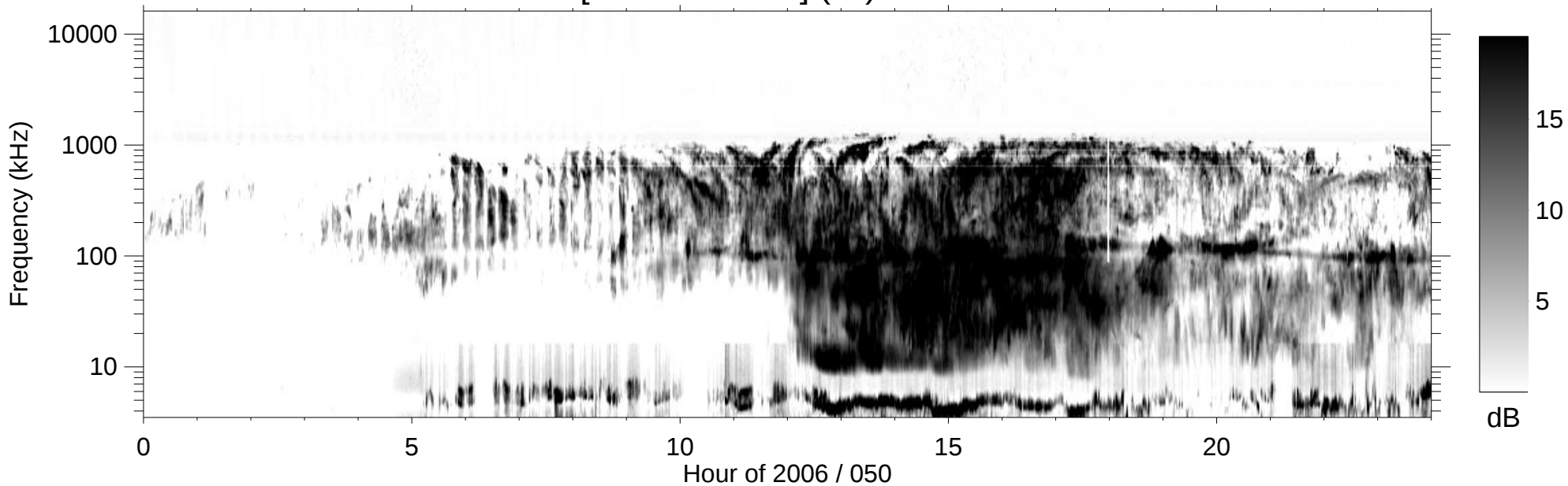
RPWS [ABCH1H2/Ex] (-B) 2006/02/19
