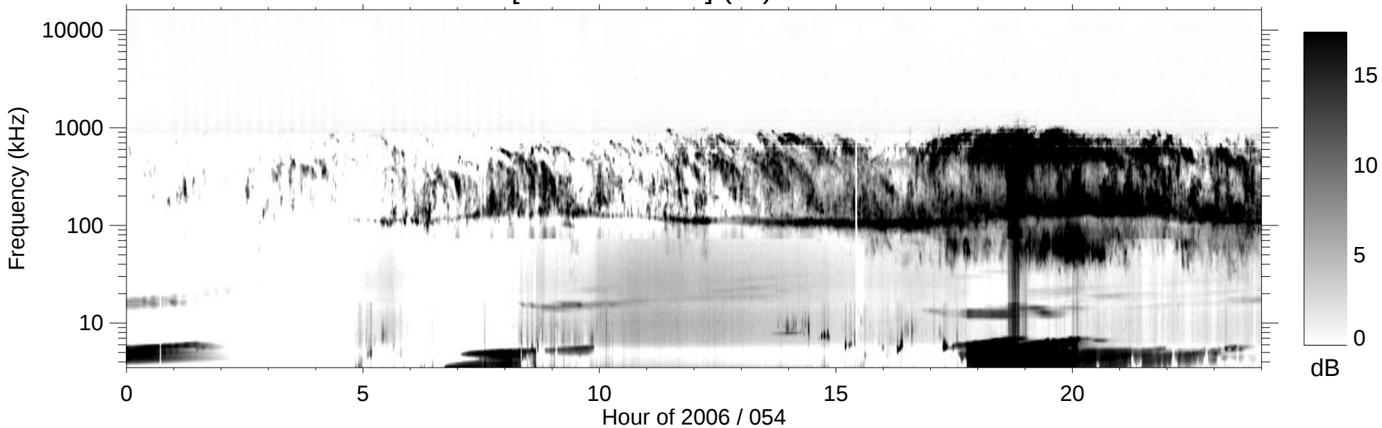
RPWS [ABCH1H2/Ex] (-B) 2006/02/23
