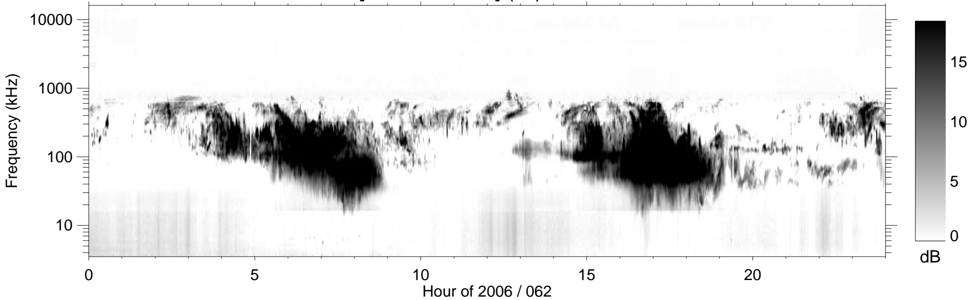
RPWS [ABCH1H2/Ex] (-B) 2006/03/03
