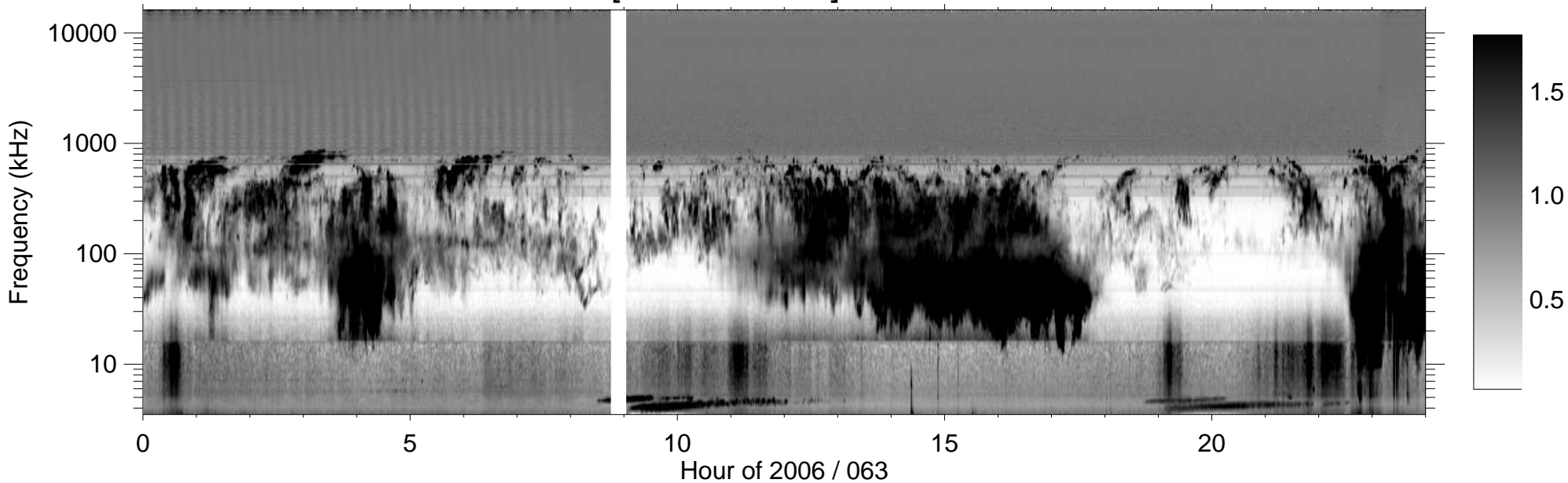
RPWS [ABCH1H2/Ex] (-B) 2006/03/04
