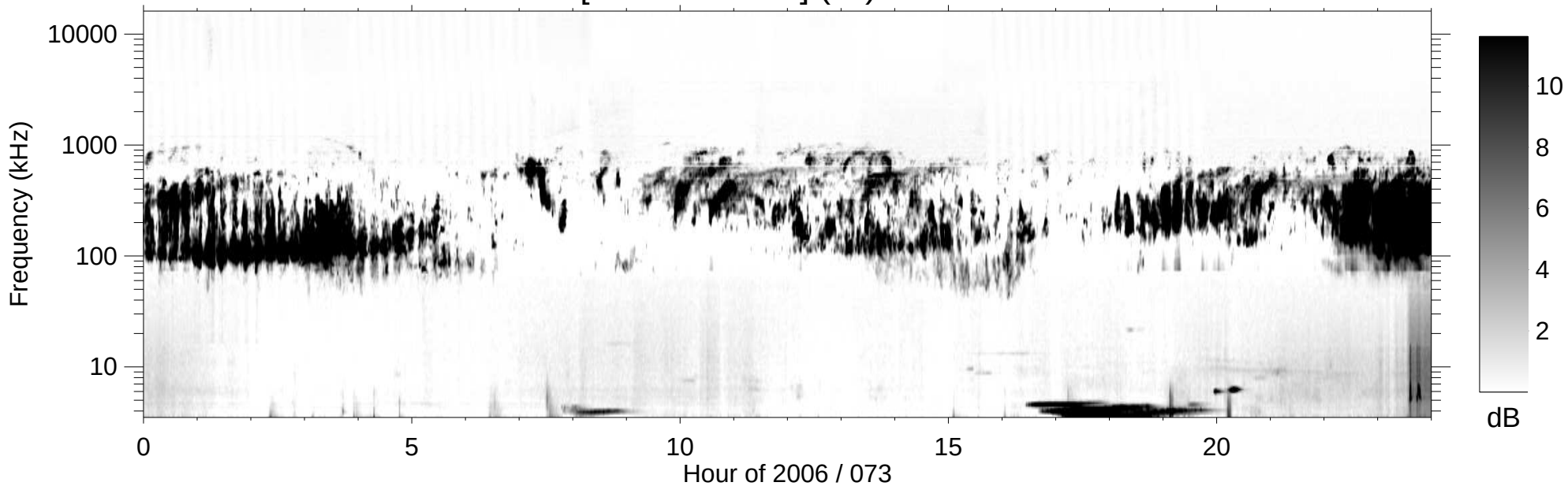
RPWS [ABCH1H2/Ex] (-B) 2006/03/14
