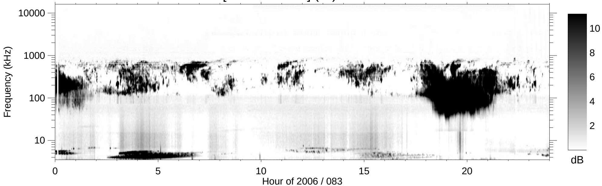
RPWS [ABCH1H2/Ex] (-B) 2006/03/24
