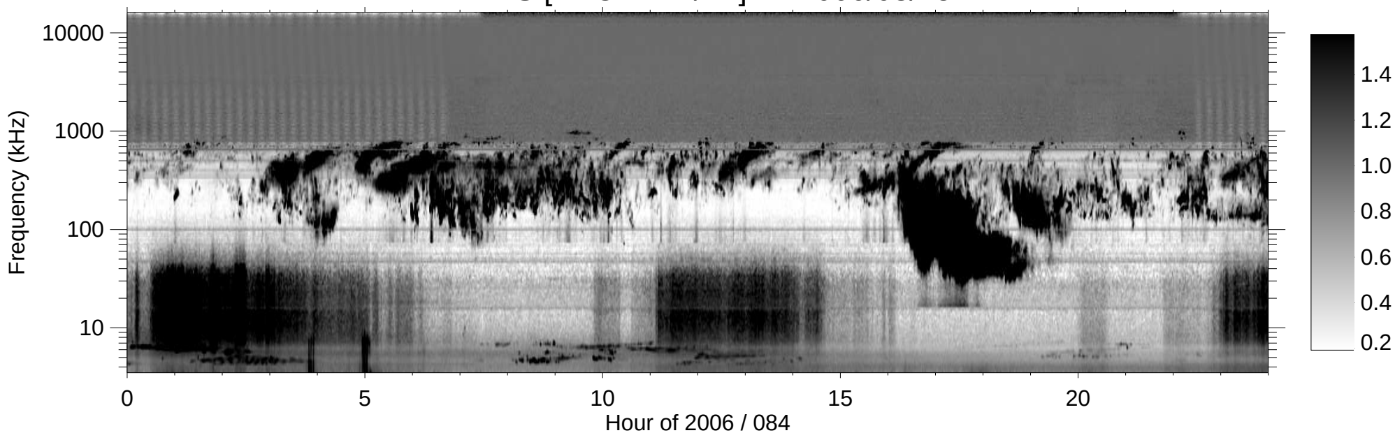
RPWS [ABCH1H2/Ex] (-B) 2006/03/25
