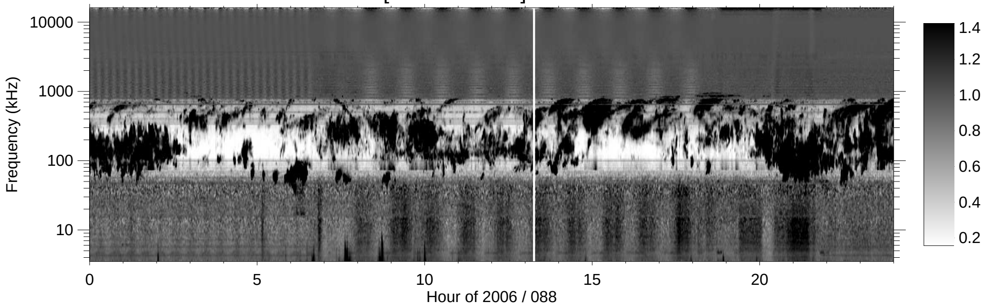
RPWS [ABCH1H2/Ex] (-B) 2006/03/29
