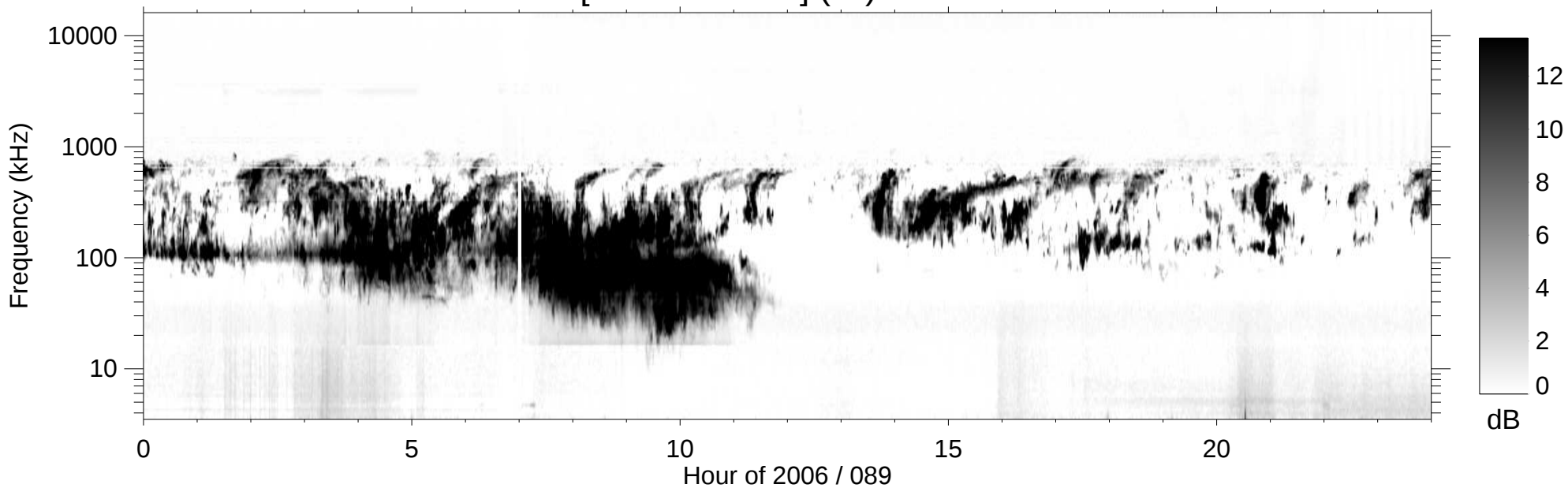
RPWS [ABCH1H2/Ex] (-B) 2006/03/30
