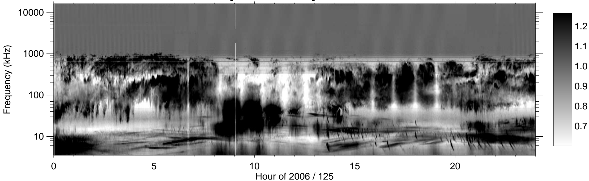
RPWS [ABCH1H2/Ex] (-B) 2006/05/05
