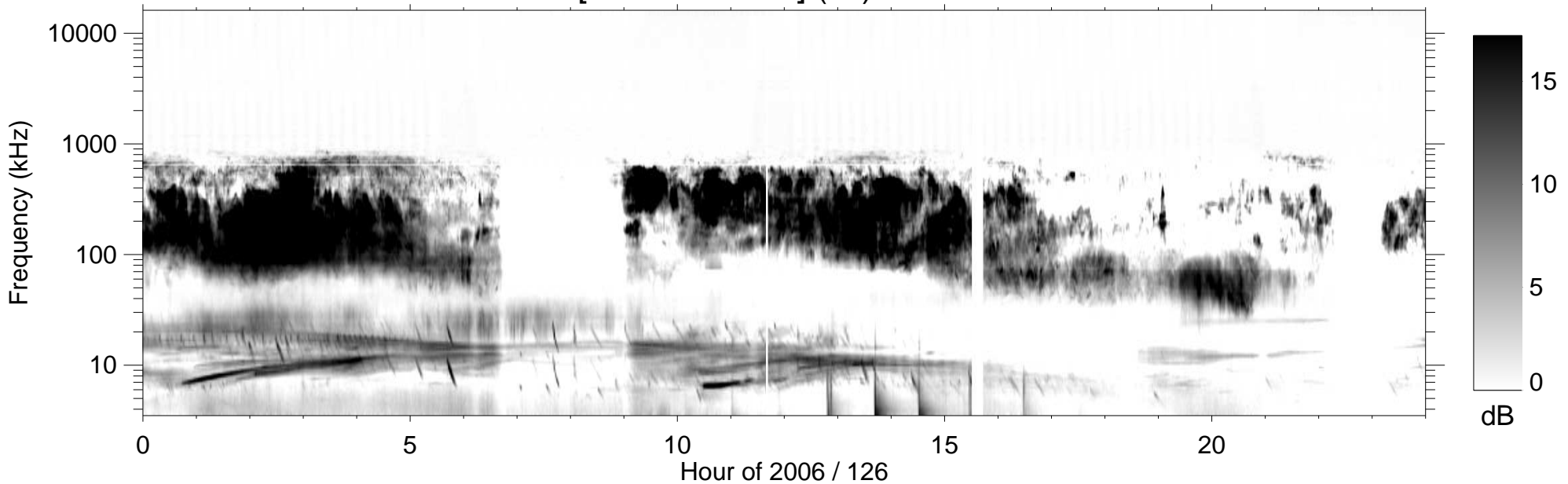
RPWS [ABCH1H2/Ex] (-B) 2006/05/06
