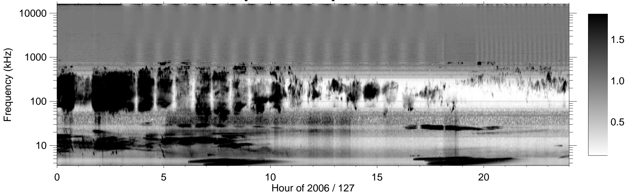
RPWS [ABCH1H2/Ex] (-B) 2006/05/07
