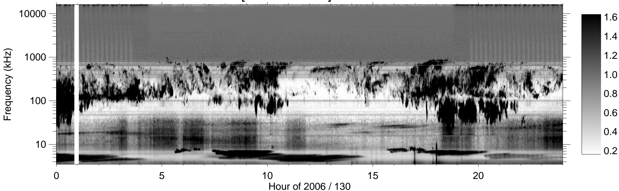
RPWS [ABCH1H2/Ex] (-B) 2006/05/10
