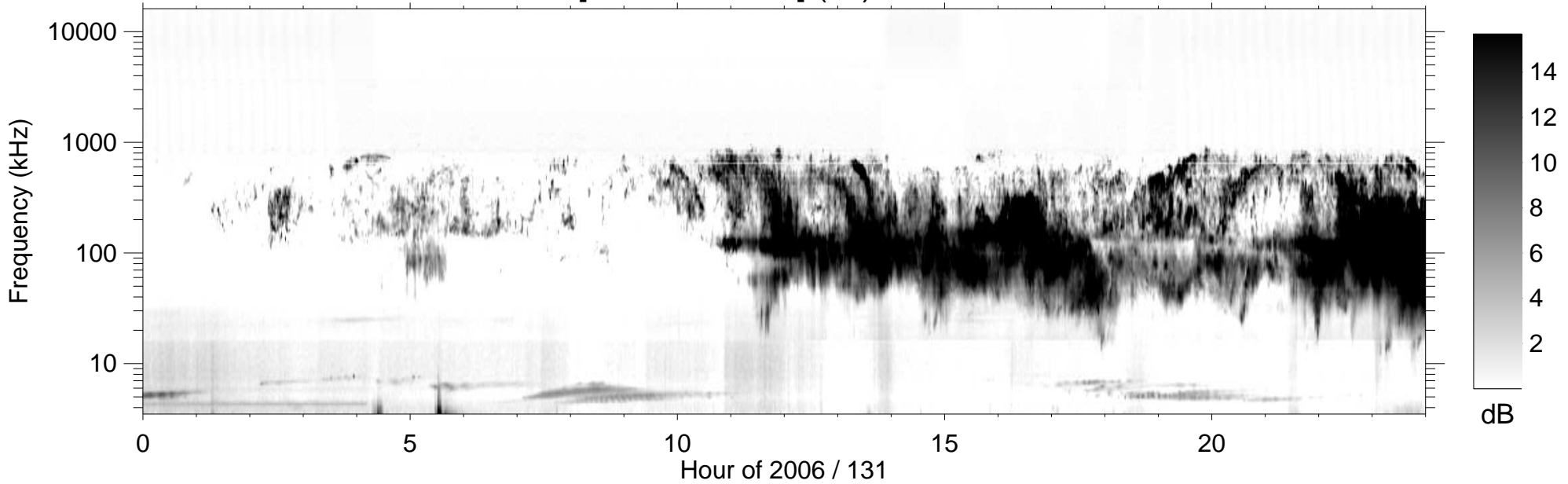
RPWS [ABCH1H2/Ex] (-B) 2006/05/11
