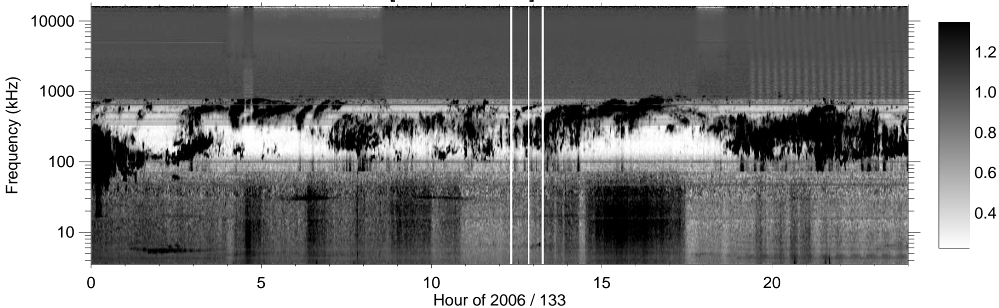
RPWS [ABCH1H2/Ex] (-B) 2006/05/13
