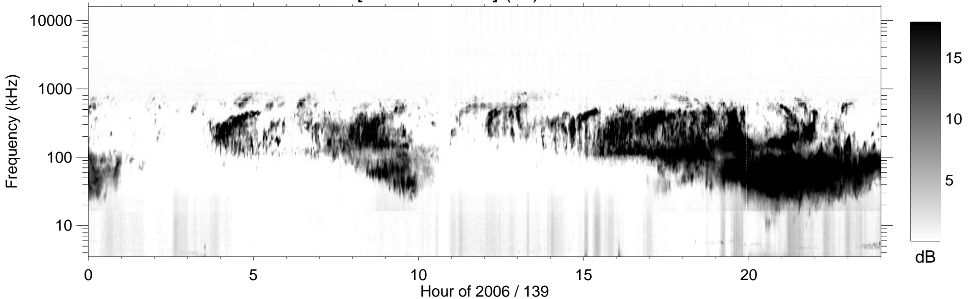
RPWS [ABCH1H2/Ex] (-B) 2006/05/19
