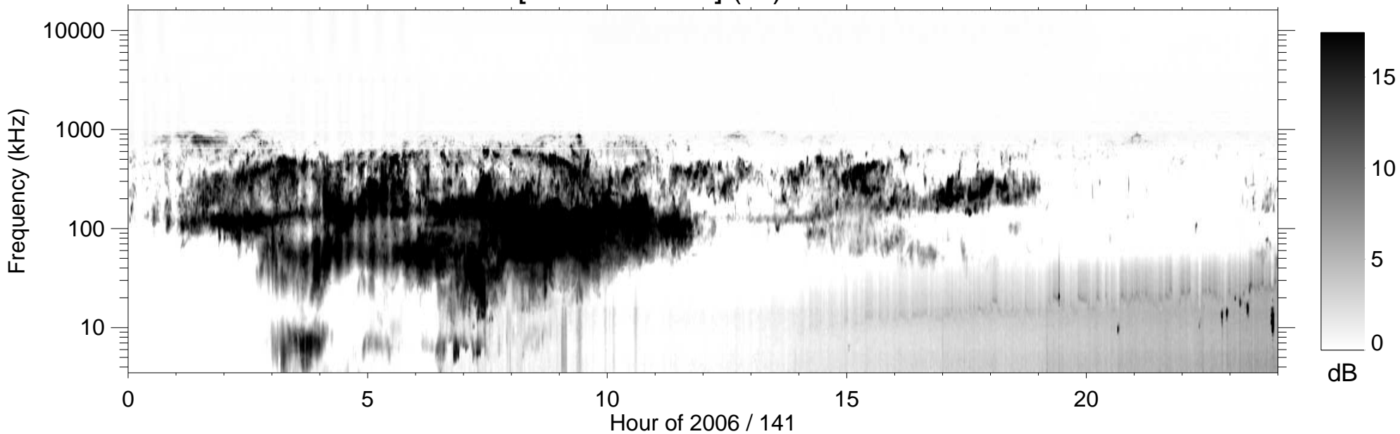
RPWS [ABCH1H2/Ex] (-B) 2006/05/21
