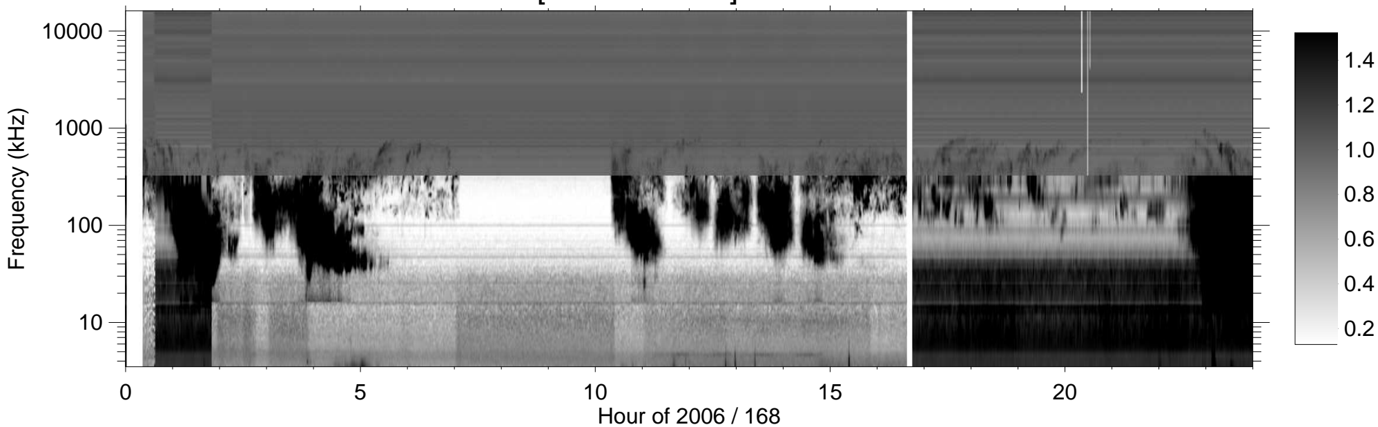
RPWS [ABCH1H2/Ex] (-B) 2006/06/17
