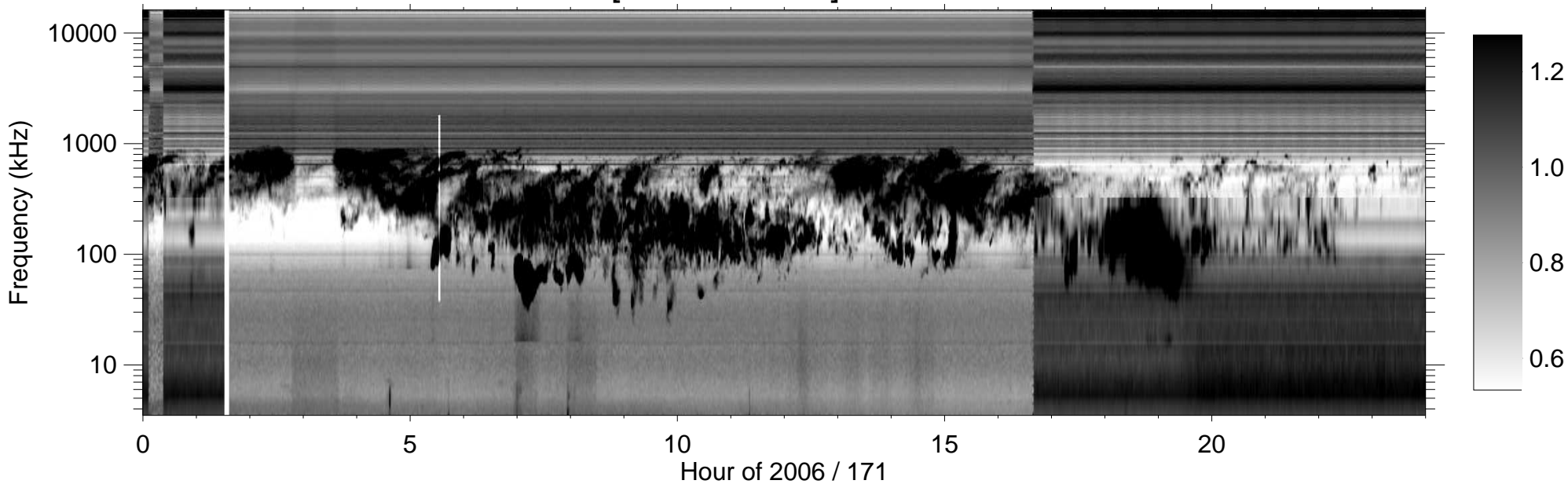
RPWS [ABCH1H2/Ex] (-B) 2006/06/20
