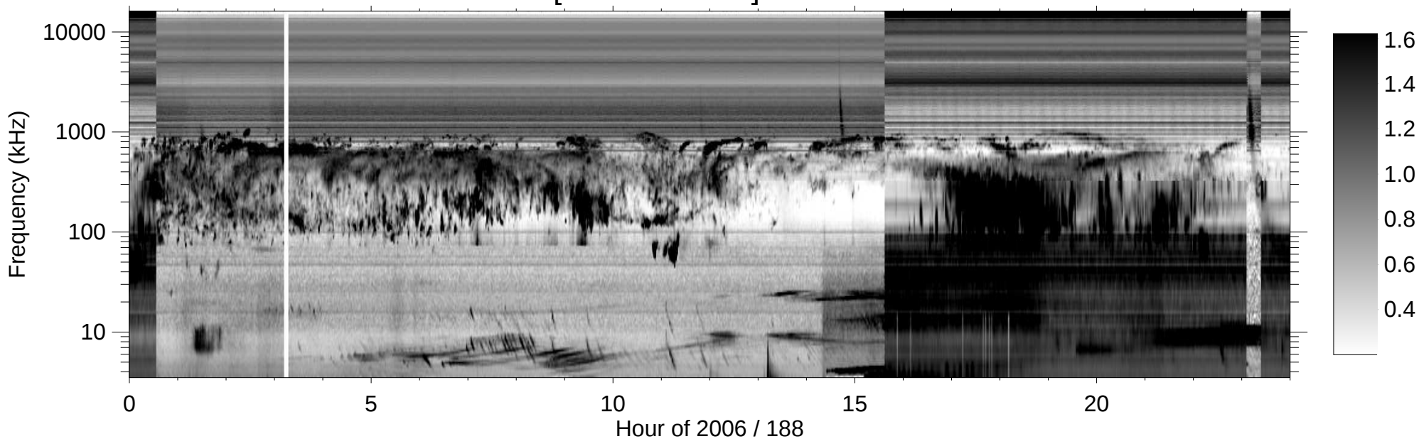
RPWS [ABCH1H2/Ex] (-B) 2006/07/07
