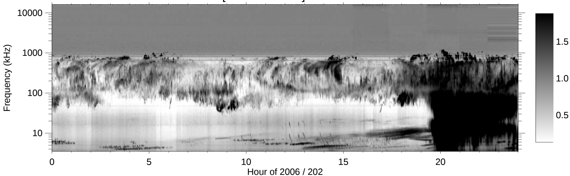
RPWS [ABCH1H2/Ex] (-B) 2006/07/21
