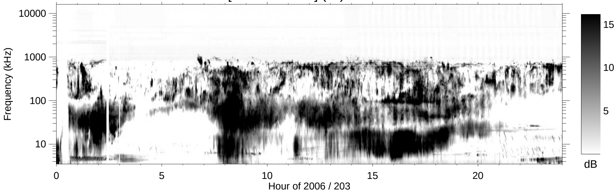
RPWS [ABCH1H2/Ex] (-B) 2006/07/22
