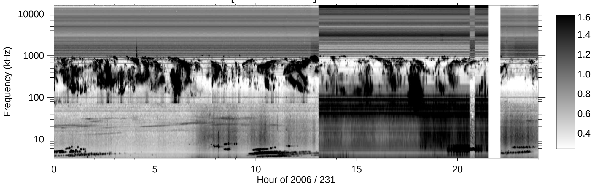
RPWS [ABCH1H2/Ex] (-B) 2006/08/19
