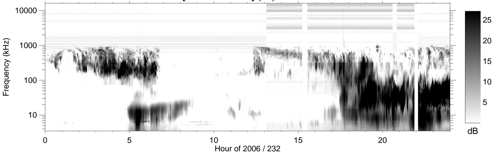
RPWS [ABCH1H2/Ex] (-B) 2006/08/20
