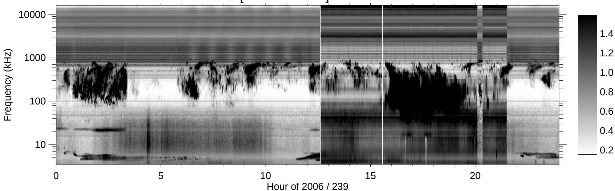
RPWS [ABCH1H2/Ex] (-B) 2006/08/27
