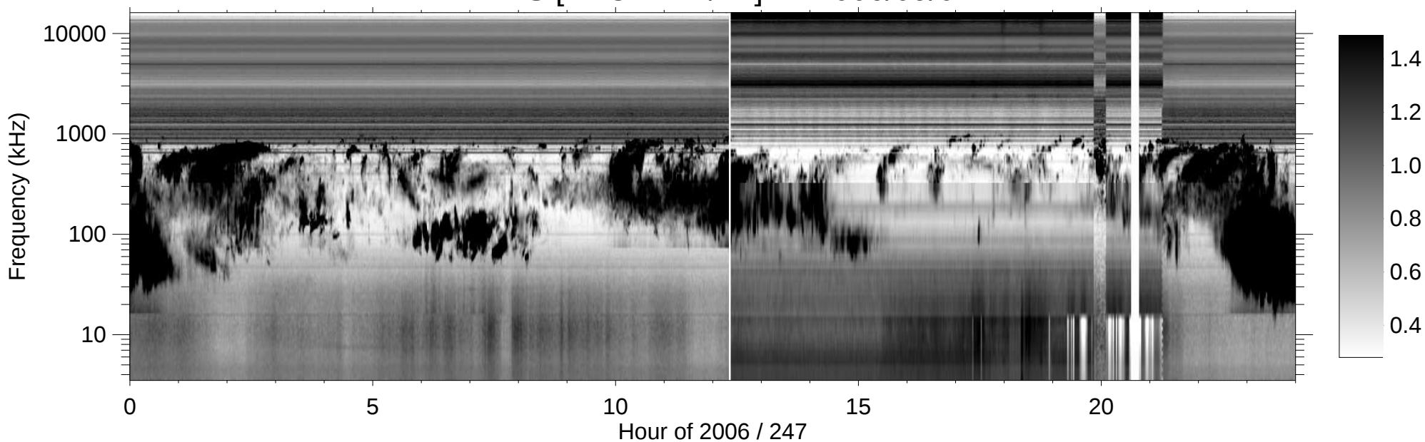
RPWS [ABCH1H2/Ex] (-B) 2006/09/04
